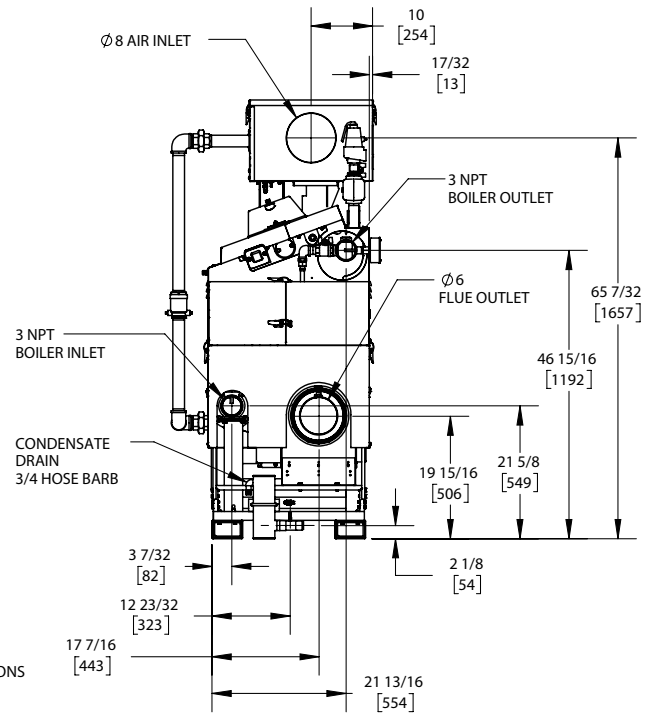
REAR VIEW
